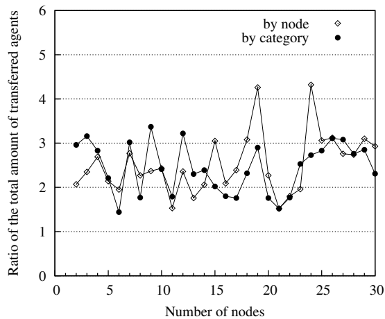
Figure 11 - Ratio of the total amount of transferred agents.
