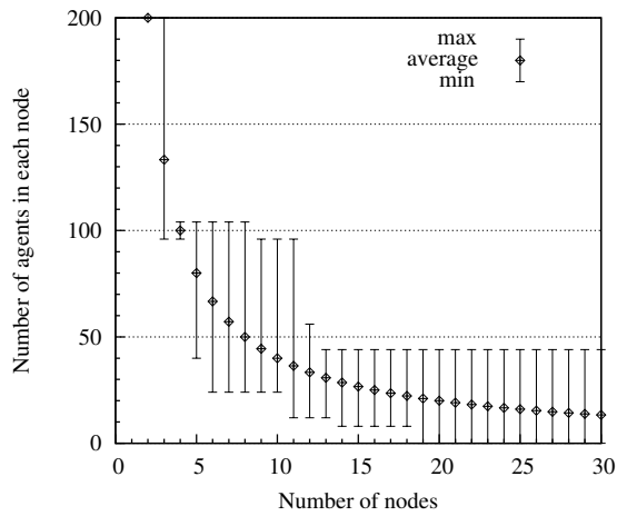
Figure 10 - The number of agents in each node with the backup and recovery scheme by category.
