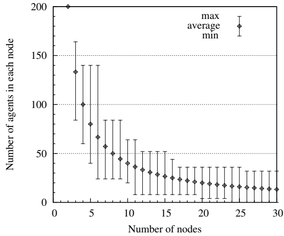
Figure 9 - The number of agents in each node with the backup and recovery scheme by node.
