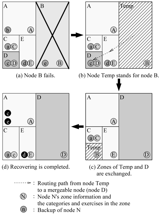
Figure 7 - Change of the P2P network when node B fails.
