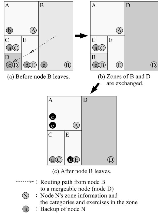
Figure 6 - Change of the P2P network with a backup and recovery scheme when node D leaves.
