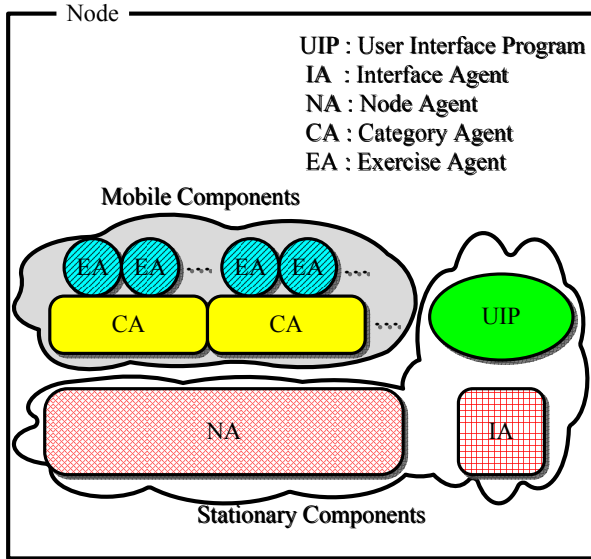
Figure 2. Architecture of a node.
