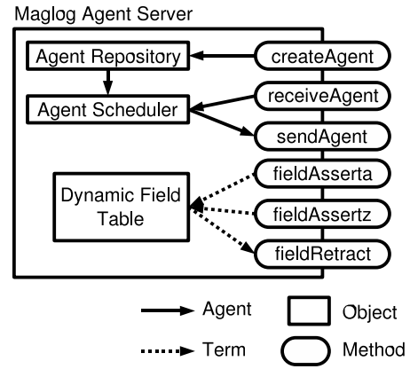
Figure 6. Structure of an agent server.
