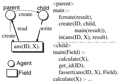
Figure 2. Agents can communicate synchronously through a field.
