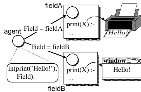
Figure 3. Dynamic Change of agent's behavior through entering a field.
