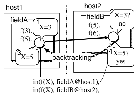
Figure 4. Backtracking and unification between two computers.
